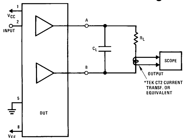
578303 FIGURE 1. Differential Connection
