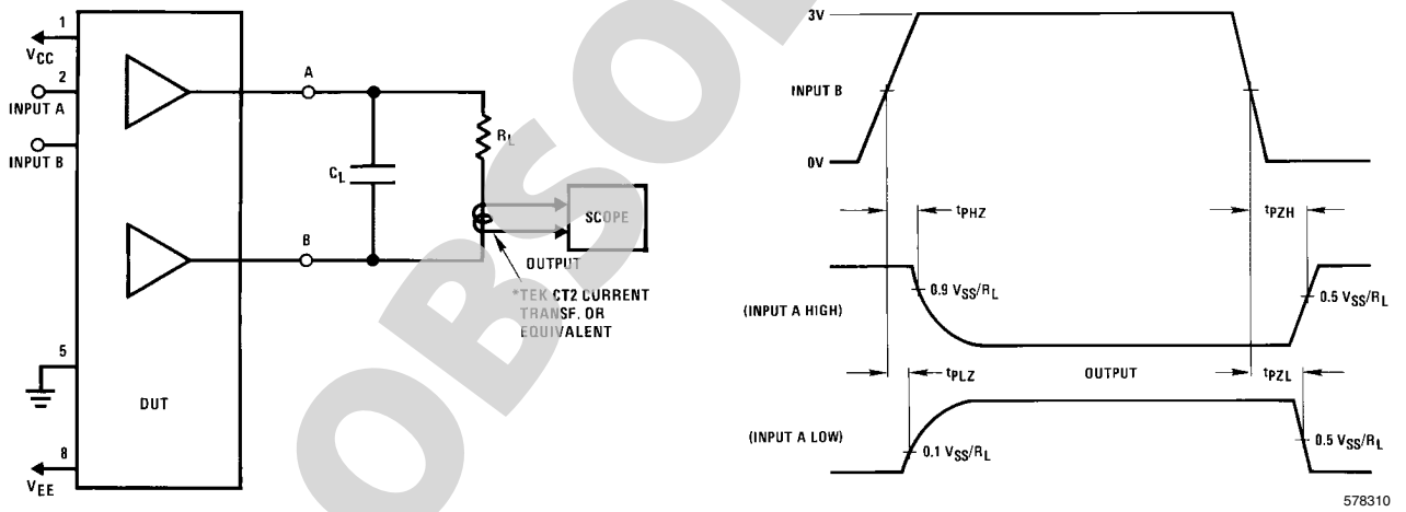
FIGURE 4. TRI-STATE Delays
